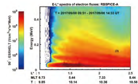
The electron zebras observed by RBSPICE instrument on-board Van Allen Probes-A on 2017/09/08.
