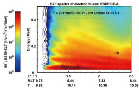
The electron zebras observed by RBSPICE instrument on-board Van Allen Probes-A on 2017/09/08.
