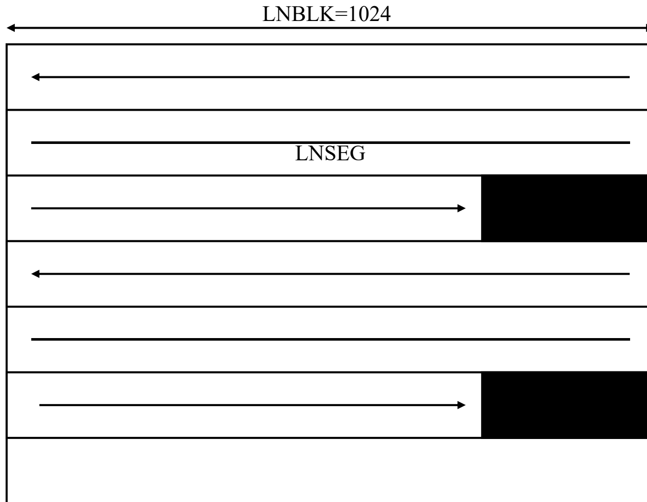
Case of longer length of segment ( LNSEG ) than the length of a data block ( LNBLK )
