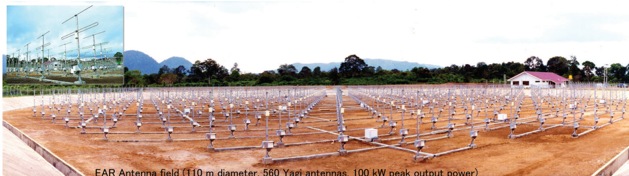
EAR Antenna field (110 m diameter, 560 Yagi antennas, 100 kW peak output power)
