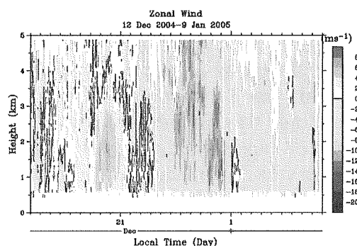
Figure 2. Time-height cross-section of zonal winds observed with SB-LTR during December 12, 2004-January 9, 2005.
