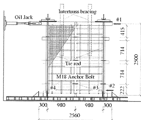
Fig3: Experimental set up and dimensions of type-A
